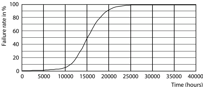
Life Expectancy Diagram - Ess LEDBulb 8-60W E27 6500K A19 10CT MX
