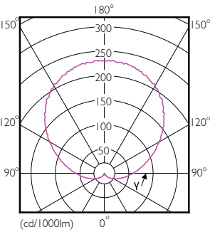
Light Distribution Diagram - Ess LEDBulb 8-60W E27 6500K A19 10CT MX
