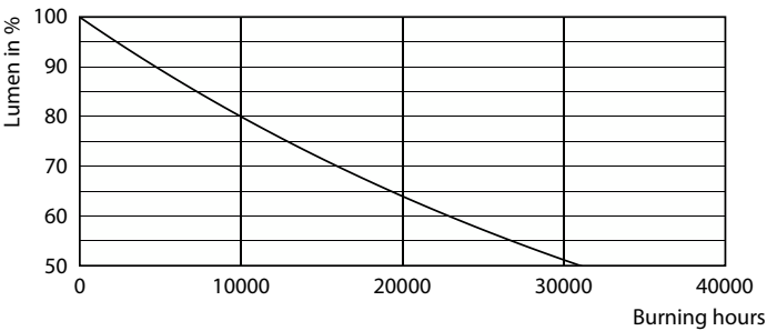
Lumen Maintenance Diagram - Ess LEDBulb 8-60W E27 6500K A19 10CT MX
