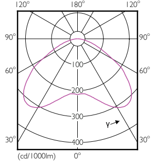
Light Distribution Diagram - TForce LED HB MV ND 200-160W E40 840 WB
