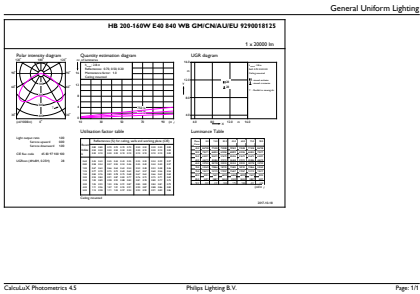
General uniform lighting - TForce Core HB 200-160W E40 840 WB RCA
