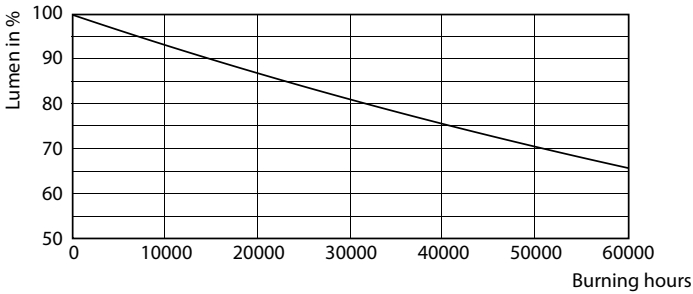
Lumen Maintenance Diagram - TForce Core HB 200-160W E40 840 WB RCA
