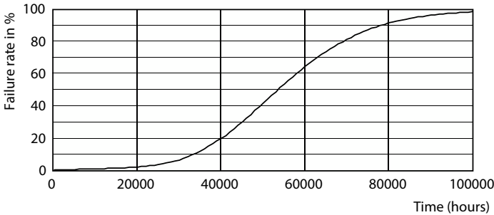
Life Expectancy Diagram - TForce Core HB 200-160W E40 840 WB RCA
