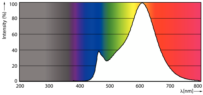
Spectral Power Distribution Colour - CLA LEDCandle ND 4-40W B35 B22 827 CL
