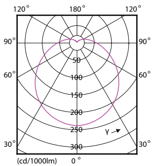
Light Distribution Diagram - CorePro LEDbulb ND 20-150W E27 865 A80
