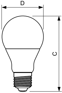
Bulb A19 120V 9.5-60W 800lm 2700K E26 D
