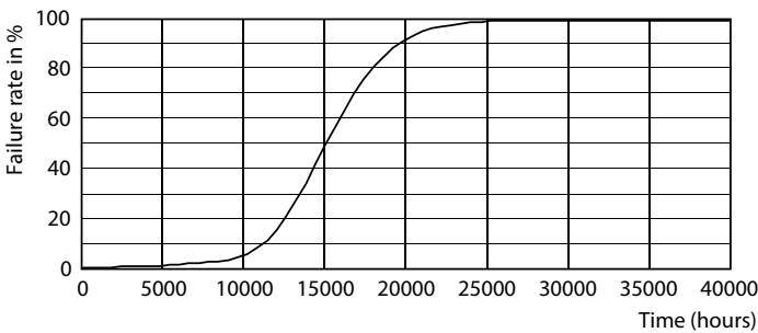
Life Expectancy Diagram - 9.5A19/PER/827/P/E26/DIM 6/1FB
