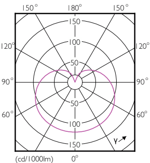
Light Distribution Diagram - 9.5A19/PER/827/P/E26/DIM 6/1FB
