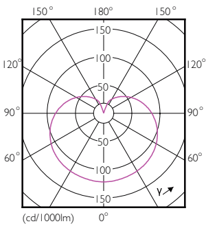
Light Distribution Diagram - 12A21/PER/850/P/E26/DIM 6/1FB
