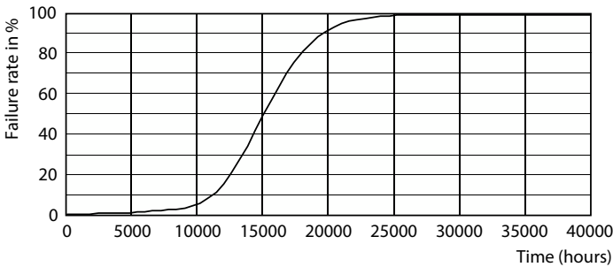
Life Expectancy Diagram - 12A21/PER/850/P/E26/DIM 6/1FB
