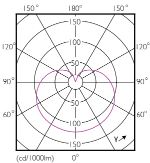
Light Distribution Diagram - 16A21/PER/850/P/E26/DIM 6/1FB
