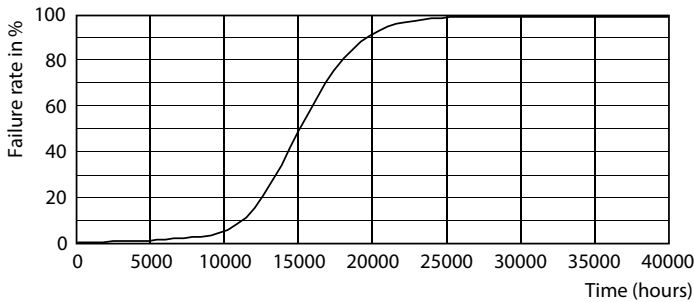
Life Expectancy Diagram - 16A21/PER/850/P/E26/DIM 6/1FB
