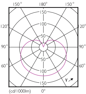
Light Distribution Diagram - 9.5A19/PER/827-22/P/E26/WG 6/1FB
