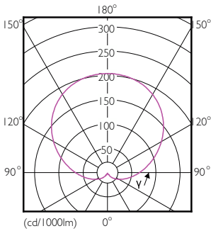
Light Distribution Diagram - LEDBulb 4.5W E27 3000K W A55 1PF/10 BR
