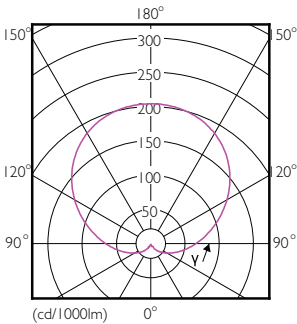
Light Distribution Diagram - LEDBulb 4.5W E27 6500K W A55 1PF/10 BR
