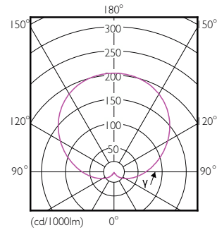
Light Distribution Diagram - LEDBulb 5W E27 6500K W A19 1BL/6 MX
