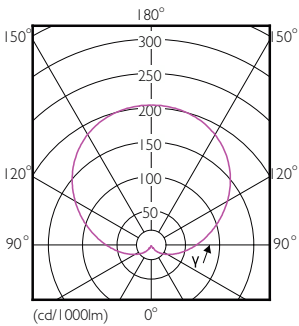
Light Distribution Diagram - LEDBulb 10W E27 3000K W A19 1PF/6 MX
