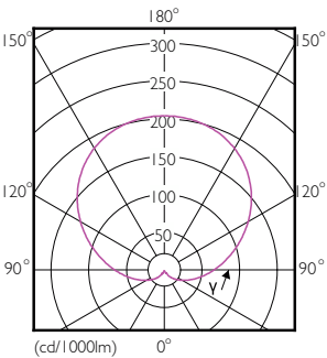
Light Distribution Diagram - LEDBulb 9.5W E27 6500K W A55 1PF/10 BR
