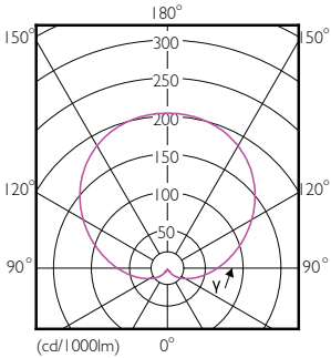
Light Distribution Diagram - LEDBulb 10W E27 6500K W A19 1BL/6 MX
