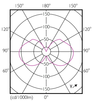
Light Distribution Diagram - 8.5A19/PER/850/CL/G/DIM 6/1CT
