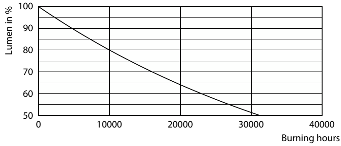
Lumen Maintenance Diagram - 4.5BA11/PER/827/CL/G/E12/DIM 6/1CT
