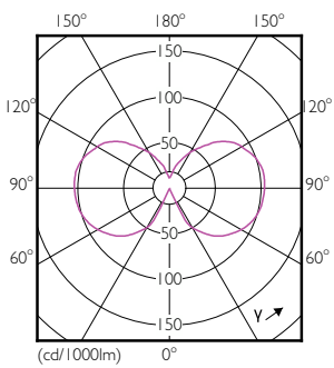
Light Distribution Diagram - 4.5BA11/PER/827/CL/G/E12/DIM 6/1CT
