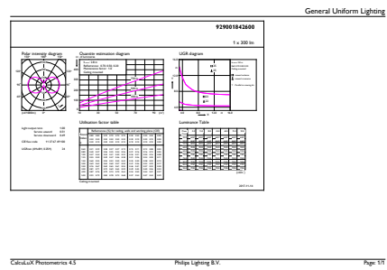
General uniform lighting - 4.5BA11/PER/850/CL/G/E12/DIM 6/1CT
