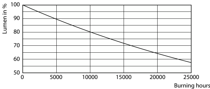
Lumen Maintenance Diagram - CorePro LEDcapsuleLV 0.9-10W G4 827
