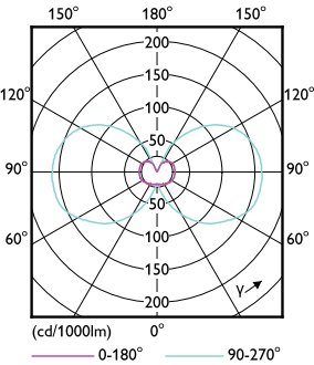
Light Distribution Diagram - CorePro LEDcapsuleLV 0.9-10W G4 827
