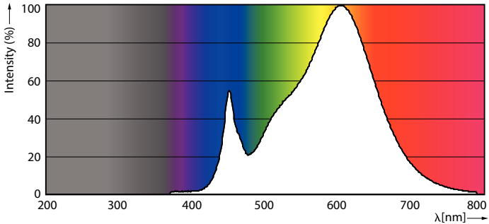
Spectral Power Distribution Colour - CorePro LEDcapsuleLV 0.9-10W G4 830
