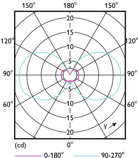
Light Distribution Diagram - CorePro LEDcapsuleLV 0.9-10W G4 830
