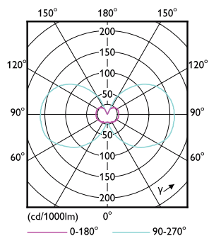
Light Distribution Diagram - CorePro LEDcapsuleLV 1.7-20W G4 827
