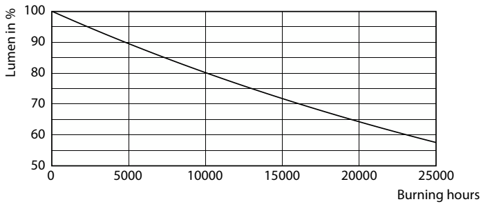
Lumen Maintenance Diagram - CorePro LEDcapsuleLV 1.7-20W G4 827
