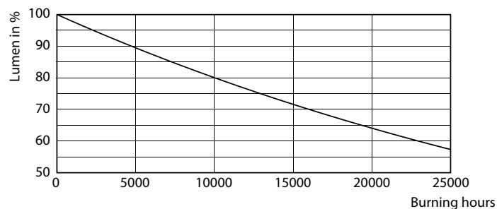
Lumen Maintenance Diagram - CorePro LEDcapsuleLV 1.7-20W GY6.35 827
