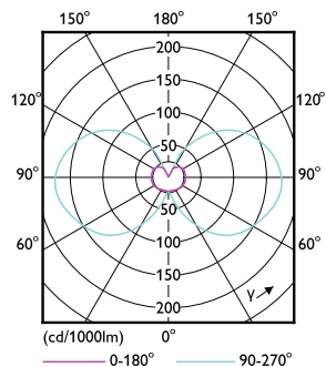
Light Distribution Diagram - CorePro LEDcapsuleLV 1.7-20W GY6.35 827
