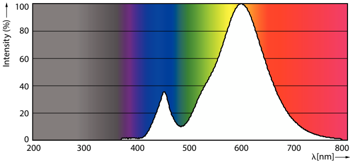
Spectral Power Distribution Colour - LED spot 5-50W 120D 2700K 220V
