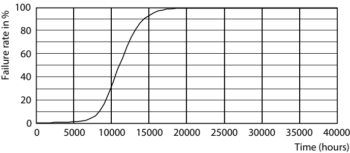
Life Expectancy Diagram - LED spot 5-50W 120D 2700K 220V
