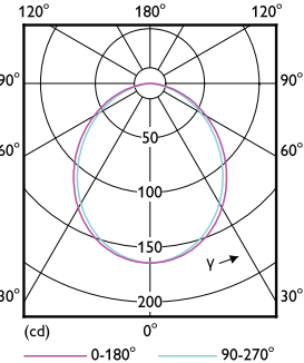
Light Distribution Diagram - LED spot 5-50W 120D 4000K 220V
