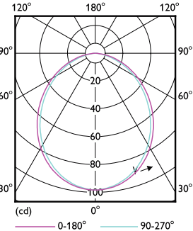
Light Distribution Diagram - LED spot 3-35W 120D 4000K 220V
