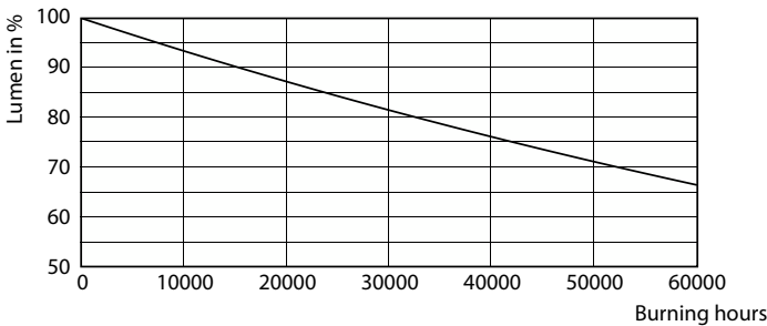
Lumen Maintenance Diagram - 14T8/COR/48-840/MF18/G 1/4 FFP
