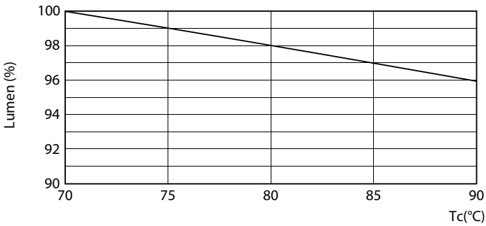
Lumen Maintenance Diagram - 14T8/COR/48-840/MF18/G 1/4 FFP
