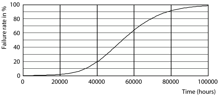
Life Expectancy Diagram - 14T8/COR/48-840/MF18/G 1/4 FFP
