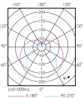
Light Distribution Diagram - 14T8/COR/48-840/MF18/G 1/4 FFP
