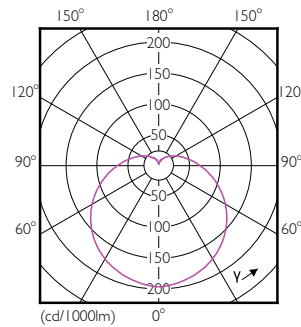
Light Distribution Diagram - 13A19/LED/865/ND 120V E27 1BC MX
