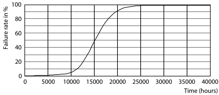
Life Expectancy Diagram - 13A19/LED/865/ND 120V E27 1BC MX
