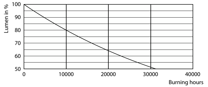
Lumen Maintenance Diagram - 13A19/LED/865/ND 120V E27 1BC MX
