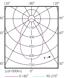
Light Distribution Diagram - 125HB/LED/750/ND NB DL BB 2/1
