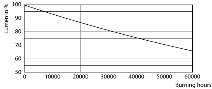
Lumen Maintenance Diagram - 125HB/LED/750/ND NB DL BB 2/1
