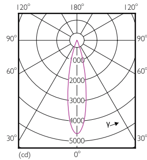
Light Distribution Diagram - 11.3PAR30S/PER/930/F25/DIM/120V 6/1FBT20
