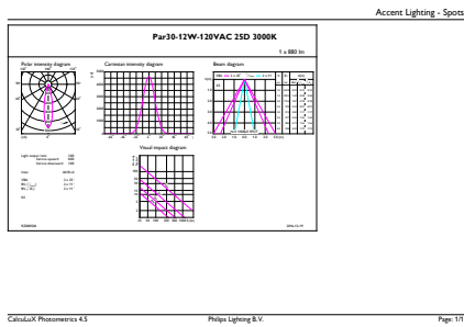
Accent Lighting Spots - 11.3PAR30S/PER/930/F25/DIM/120V 6/1FBT20
