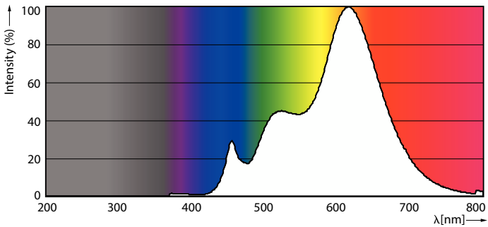
Spectral Power Distribution Colour - 6.5MR16/LED/F25/927/D/EC/12V T20 10/1FB
