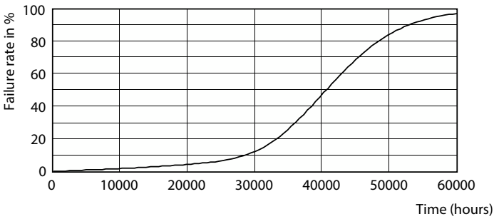
Life Expectancy Diagram - 6.5MR16/LED/F25/927/D/EC/12V T20 10/1FB
