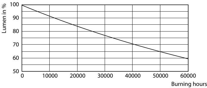
Lumen Maintenance Diagram - 6.5MR16/LED/F25/927/D/EC/12V T20 10/1FB
