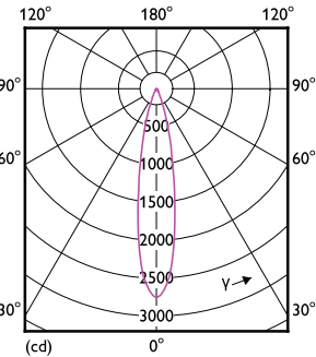
Light Distribution Diagram - 6.5MR16/LED/F25/927/D/EC/12V T20 10/1FB
