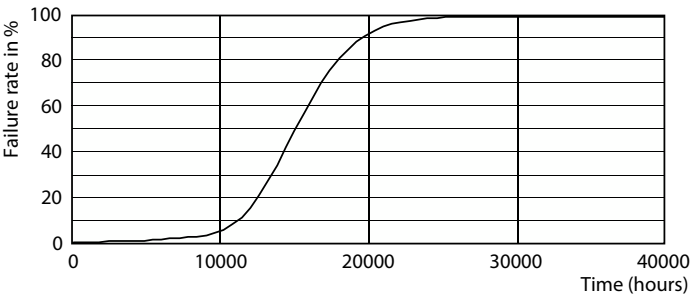
Life Expectancy Diagram - ESS LED 7W E27 2700K 230V R63
