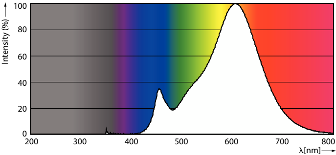
Spectral Power Distribution Colour - ESS LED 7W E27 2700K 230V R63
