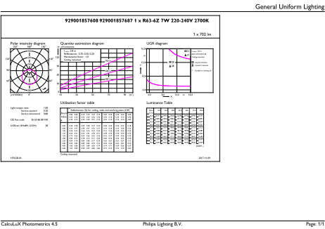
Accent Lighting Spots - ESS LED 7W E27 2700K 230V R63
