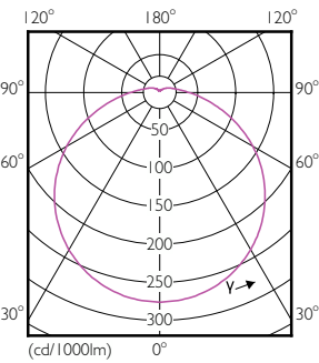
Light Distribution Diagram - LED Spot 7W E27 2700K 230V R63 RCA
