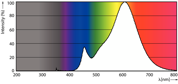
Spectral Power Distribution Colour - LED Spot 7W E27 2700K 230V R63 RCA
