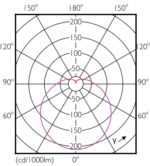
Light Distribution Diagram - LED Spot 7W E27 6500K 230V R63 RCA
