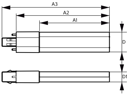
PLED PLS 120-277V 5-13W 580lm 3500K GX23
