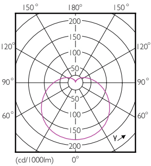
Light Distribution Diagram - LEDBulb 21W E27 6500K W A30 1PF/6 MX
