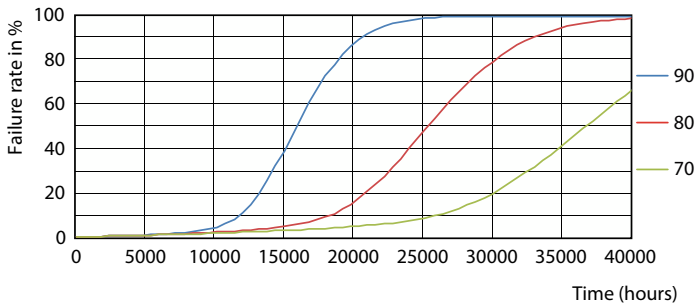
Life Expectancy Diagram - LEDBulb 21W E27 6500K W A30 1PF/6 MX
