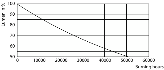
Lumen Maintenance Diagram - LEDBulb 21W E27 6500K W A30 1PF/6 MX
