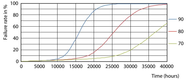
Life Expectancy Diagram - LEDBulb 19W E27 6500K W A97 1PF/6 BR
