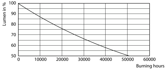
Lumen Maintenance Diagram - LEDBulb 19W E27 6500K W A97 1PF/6 BR
