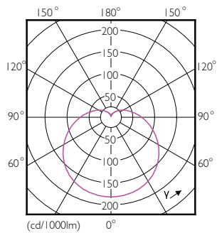
Light Distribution Diagram - LEDBulb 19W E27 6500K W A97 1PF/6 BR
