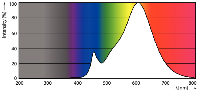
Spectral Power Distribution Colour - CorePro LEDbulb D 13.5-100W A60 E27 827
