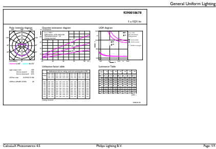
General uniform lighting - CorePro LEDbulb D 13.5-100W A60 E27 827
