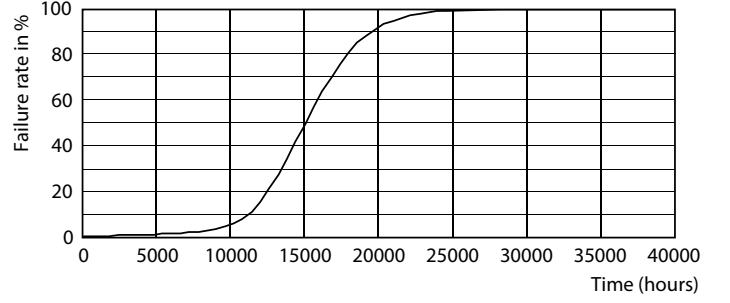
Life Expectancy Diagram - CorePro LEDbulb D 13.5-100W A60 E27 827
