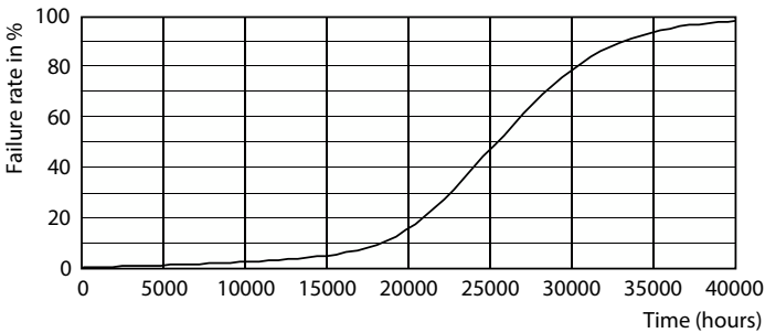
Life Expectancy Diagram - 7.8MR16/PER/930/F25/Dim/EC/12V 10/1FB
