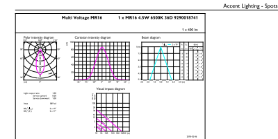
Light Distribution Diagram - ESS LED MR16 4.5-50W 36D 865 SO 100-240V
