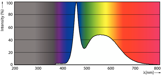
Spectral Power Distribution Colour - TForce HB 100-85W E40 865 120D GM
