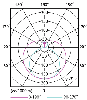
Light Distribution Diagram - 12T8/MAS/48-835/MF17/G 10/1
