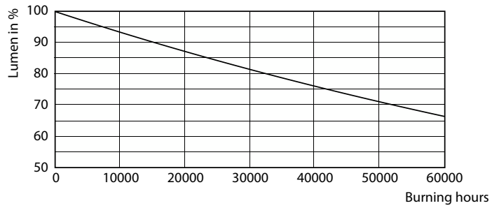
Lumen Maintenance Diagram - 12T8/MAS/48-835/MF17/G 10/1
