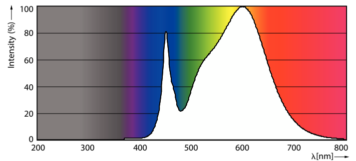
Spectral Power Distribution Colour - 12T8/MAS/48-835/MF17/G 10/1
