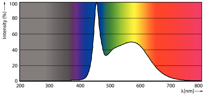
Spectral Power Distribution Colour - MAS LEDtube Sensor 1500mm HO 24W865 T8
