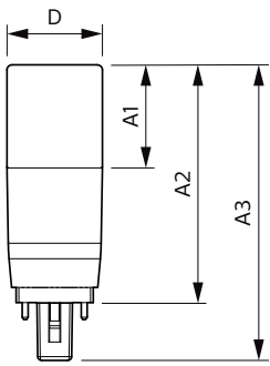
PLED PLC 7.5-13W 800lm 6500K G24d
