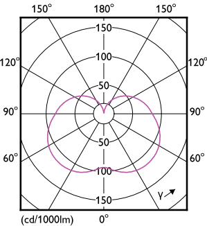
Light Distribution Diagram - LED PLC 7.5W 865 2P G24d
