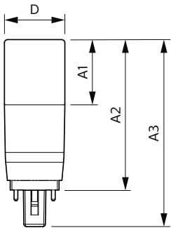
PLED PLC 11.5-18W 950lm 3000K G24d
