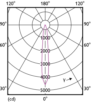
Light Distribution Diagram - MASTER LED 7-50W 930 MR16 10D Dim
