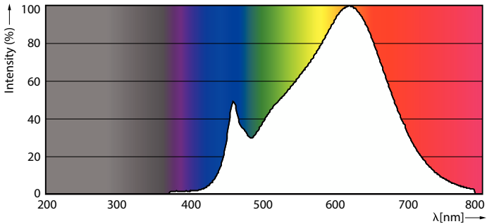
Spectral Power Distribution Colour - MASTER LED 7-50W 930 MR16 10D Dim
