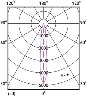
Light Distribution Diagram - MASTER LED 7-50W 940 MR16 10D Dim CN
