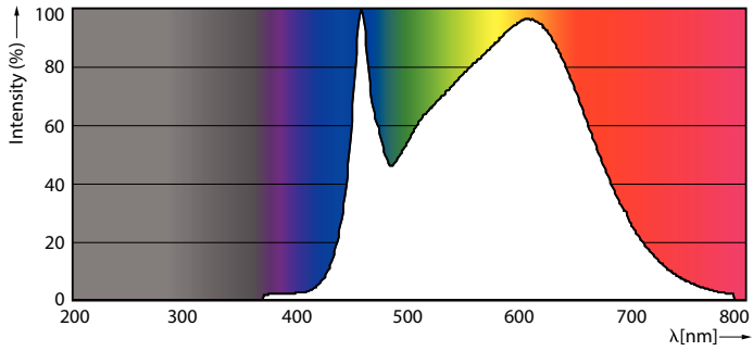
Spectral Power Distribution Colour - MASTER LED 7-50W 940 MR16 10D Dim CN
